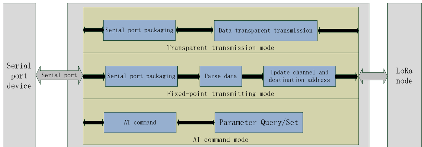
Figure 3 Functional diagram
