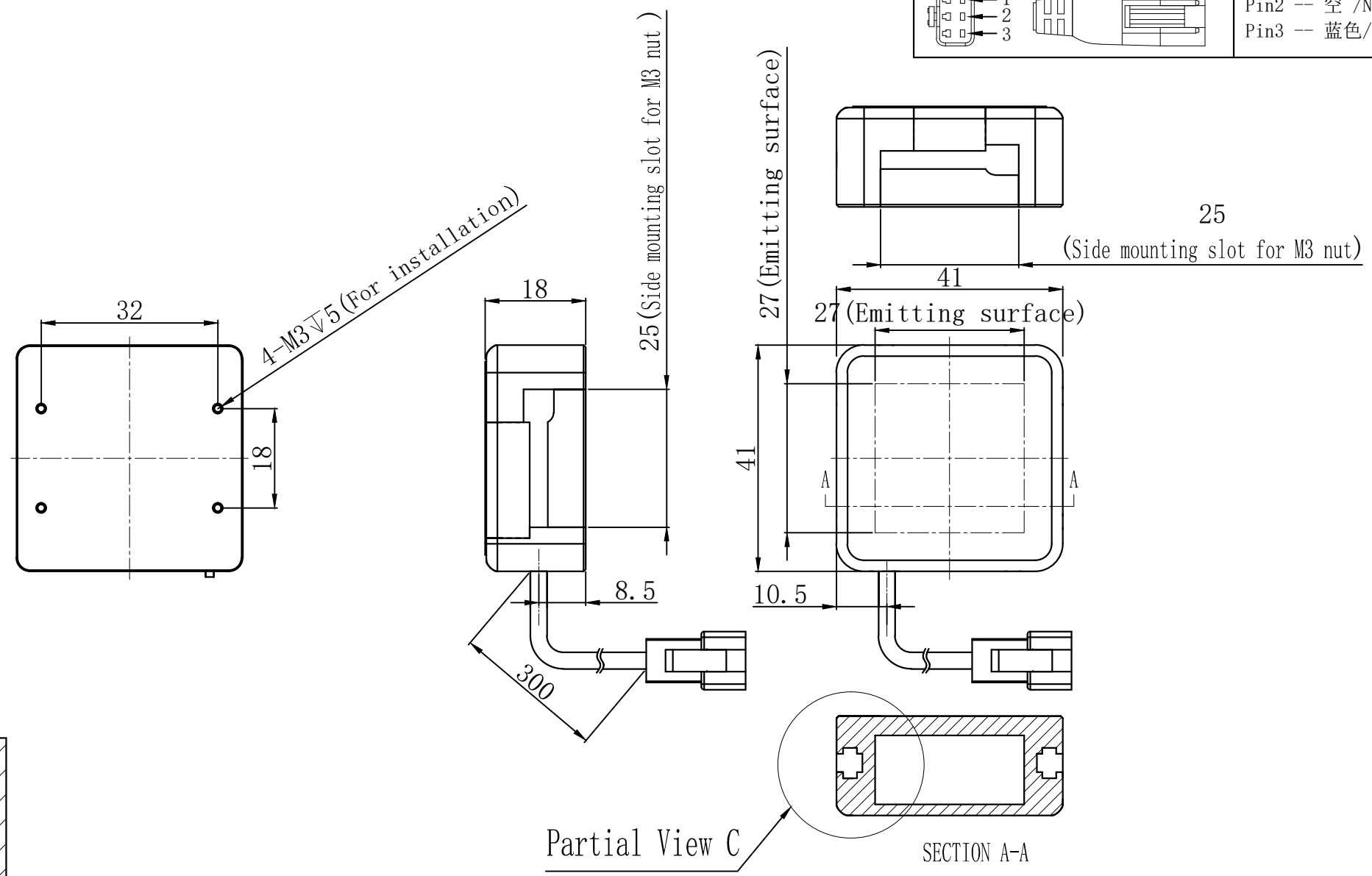
Partial View C , Four sides, Mounting slot for M3 nut, Scale 2:1
