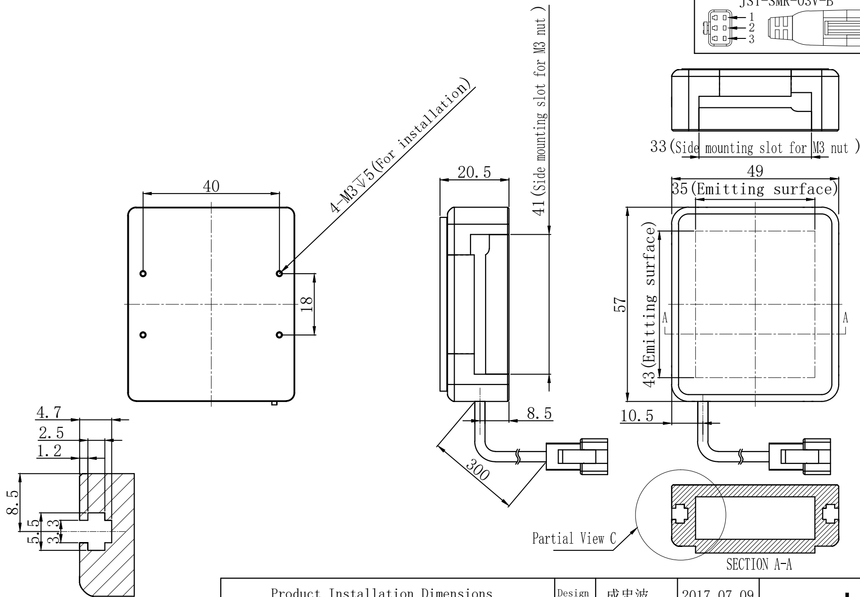
Partial View C, Four sides, Mounting slot for M3 nut, Scale 2:1
