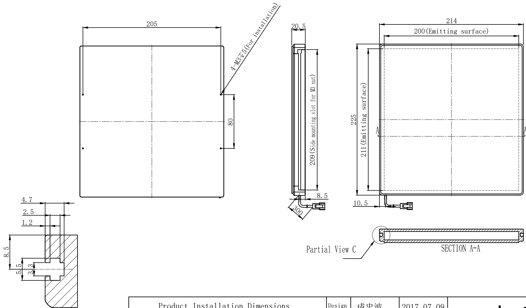
Partial View C, Four sides, Mounting slot for M3 nut, Scale 4:1
