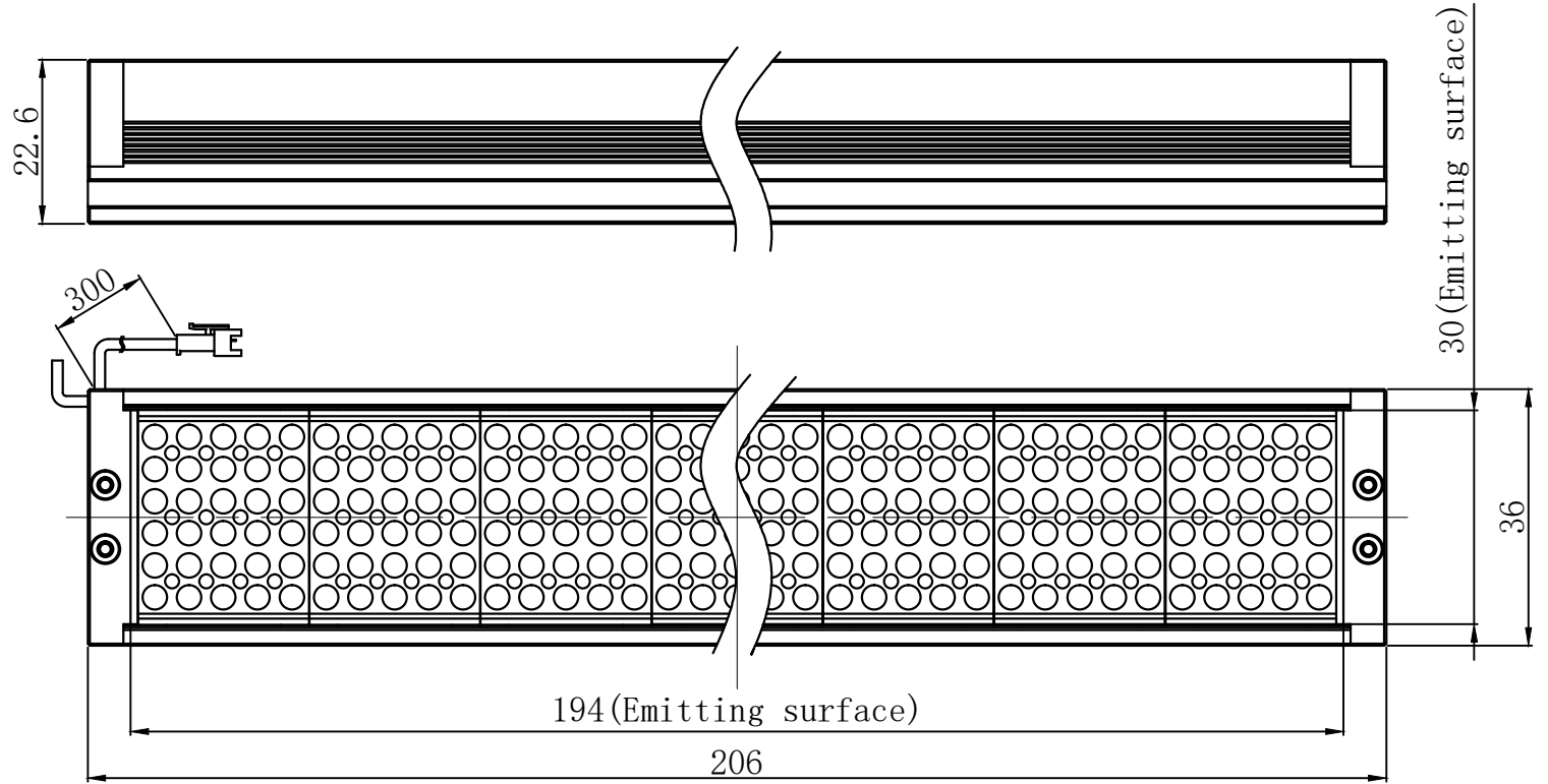
Partial view A
