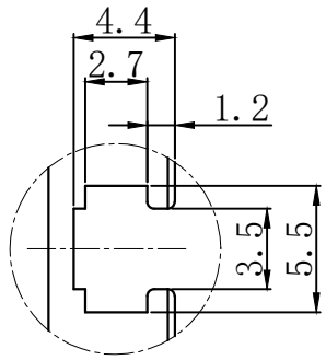
Partial view A, Scale 3:1, mounting slot for M3 nut
