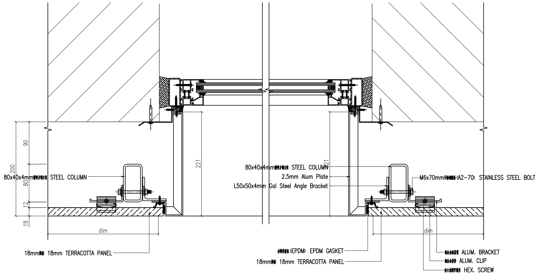
HORIZONTAL JOINT DRAWING
