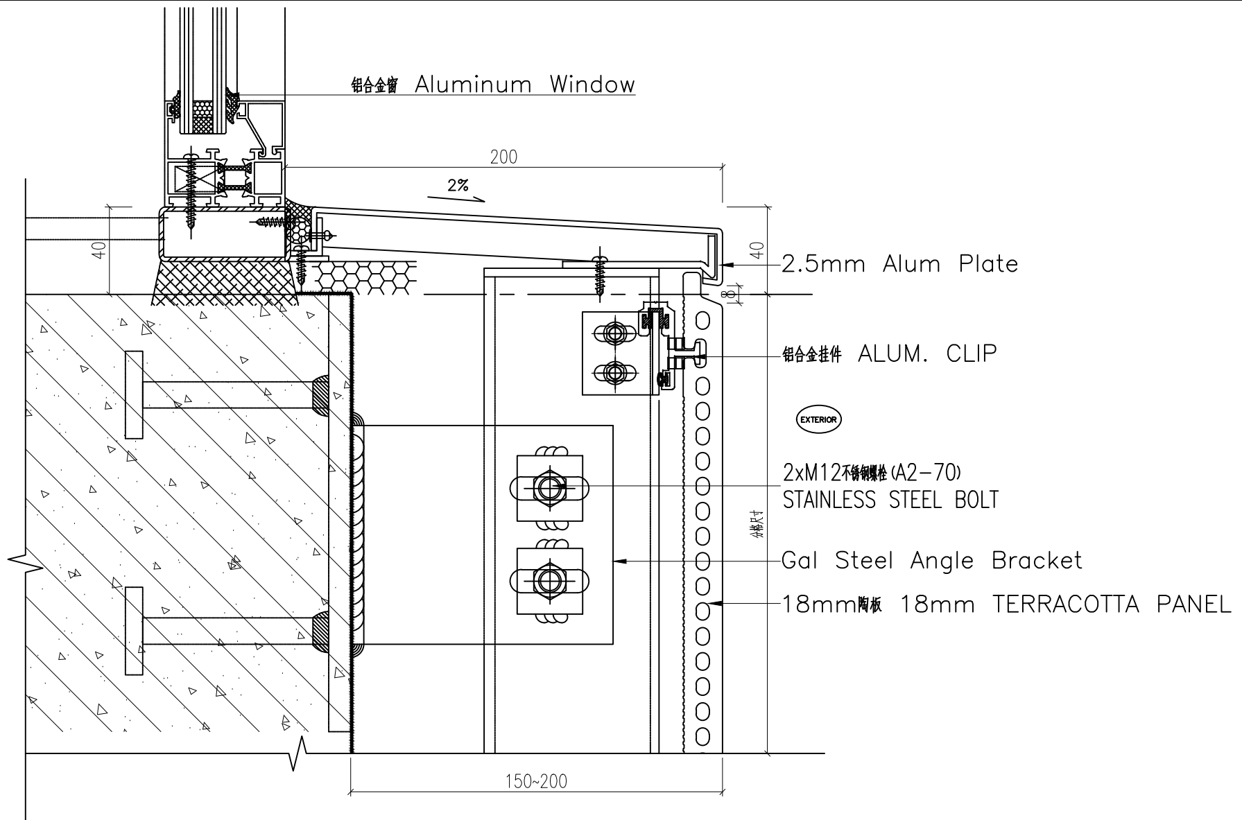
VERTICAL JOINT DRAWING
