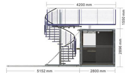
D Elevation
