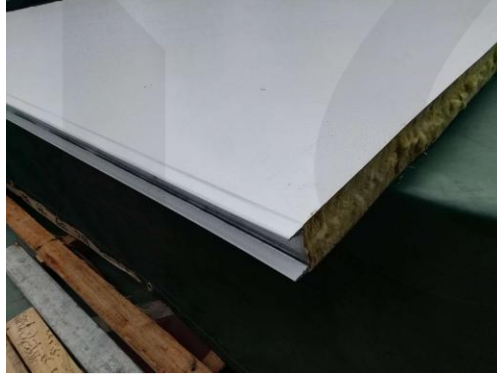
External wall panel (50mm rock wool sandwich panel)
