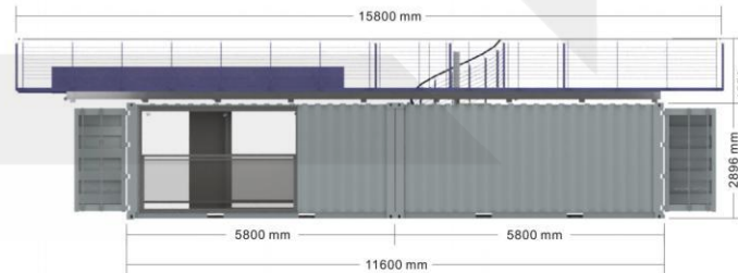
C Elevation
